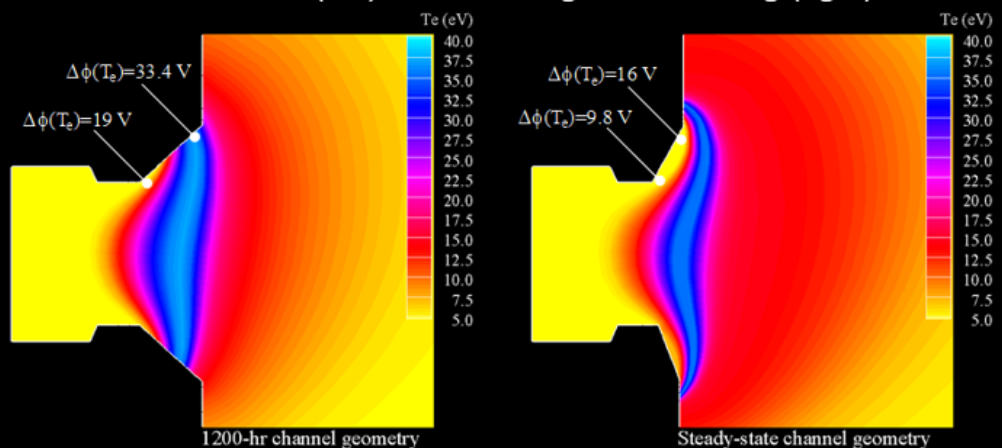
JPL numerical simulation of the electron temperature in the BPT-4000 without (left) and with magnetic shielding (right)
