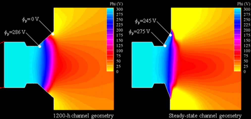
JPL numerical simulation of the plasma potential in the BPT-4000 without (left) and with magnetic shielding (right)
