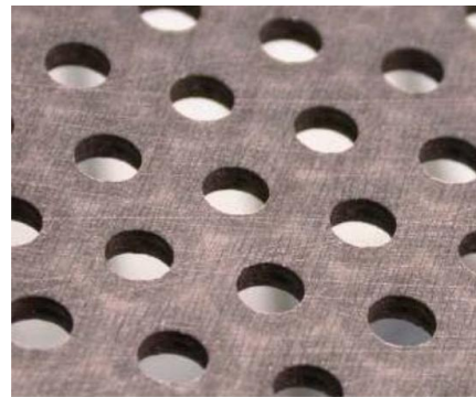
Figure 16. Post-Test Inspection Photograph of Upstream Surface of Accelerator Grid. Note pristine, un-arced condition of surface.
